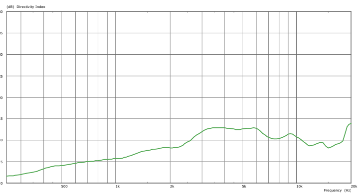
Fig. 5: Directivity index
