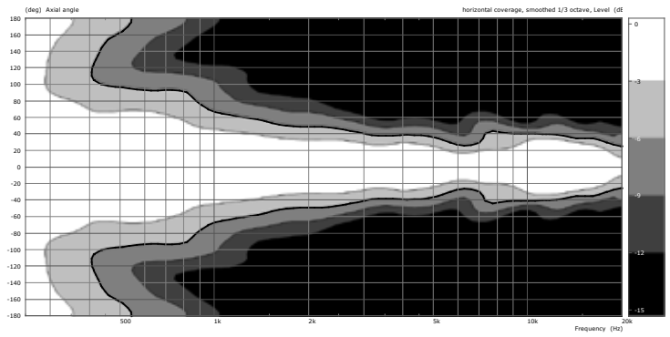
Fig. 2: Horizontal coverage
