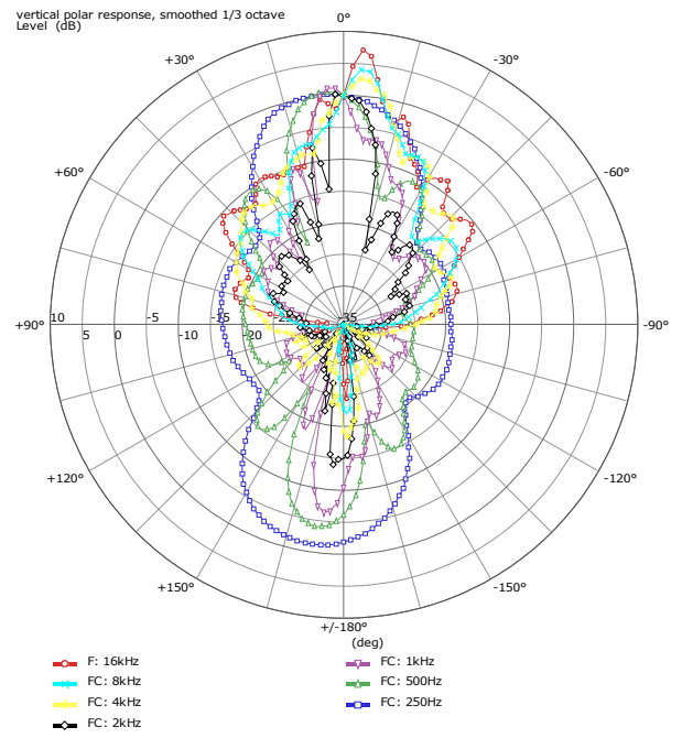
Abbildung 2: LX-220 Vertical polar response
