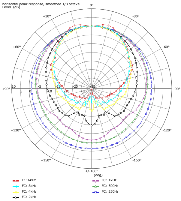
Abbildung 1: LX-220 Horizontal polar response
