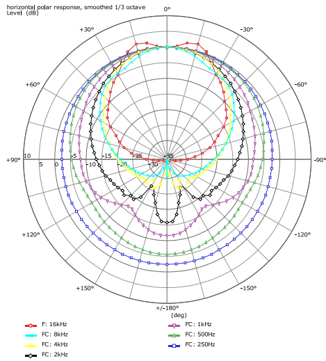
Abbildung 1: AT-061 Horizontal polar response
