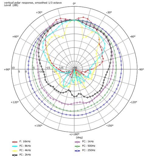
Abbildung 2: AT-061 Vertical polar response
