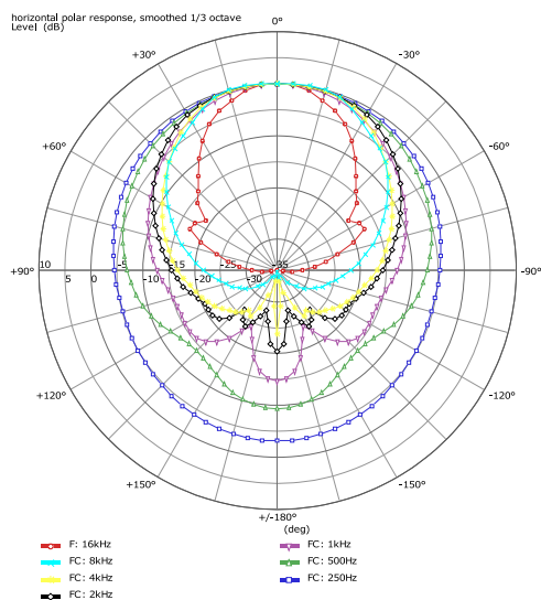
Abbildung 1: AT-201 90x60 Horizontal polar response
