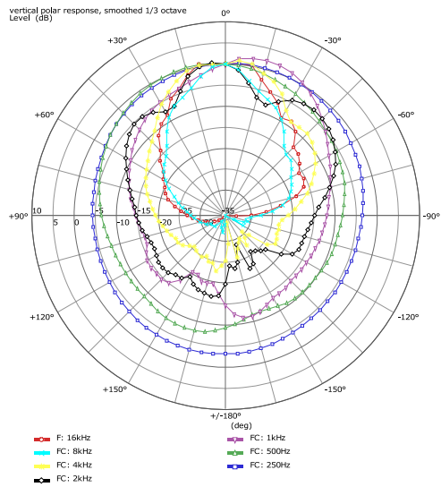
Abbildung 1: AT-201 60x40 Vertical polar response
