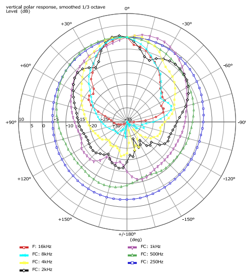
Abbildung 2: AT-201 90x60 Vertical polar response
