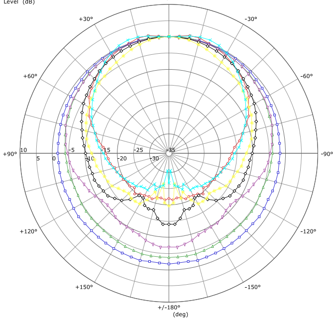
horizontal polar response, smoothed 1/3 octave Level (dB)
