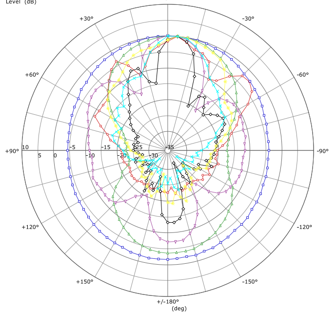
vertical polar response, smoothed 1/3 octave Level (dB)
